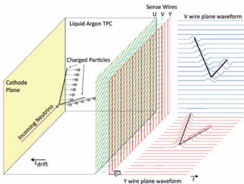
Figure 2. Schematic of the MicroBooNE liquid argon Time Projection Chamber. Ionization electrons produced by the passage of charged particles are drifted to wires planes, where their electrical signals are recorded. These detectors are optimal for neutrino interactions in the GeV regime.
